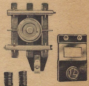
No. 37 Uncoupling Track Set—Includes uncoupling unit, No. 90 Controller. Uncouples cars equipped with magnetic couplers; operates cars with plunger-activated mechanism.
